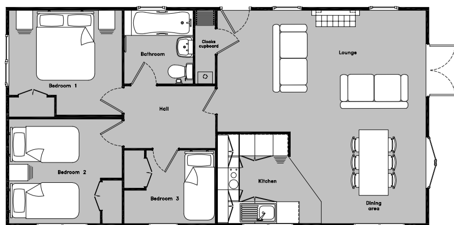
Overall size: 38 x 20ft (11.59 x 6.10m) Gross Internal Area: 760sqft (70.70sqm)
